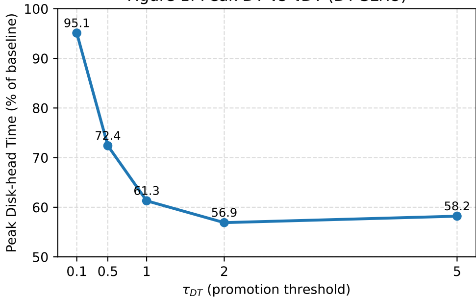
Figure 1: Peak DT vs \tau_{DT} (DT-SLRU)
